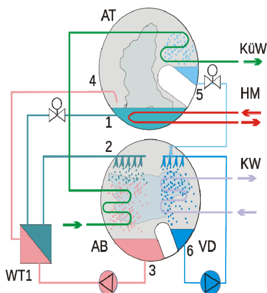
Figure 1. Solar refrigeration system.
